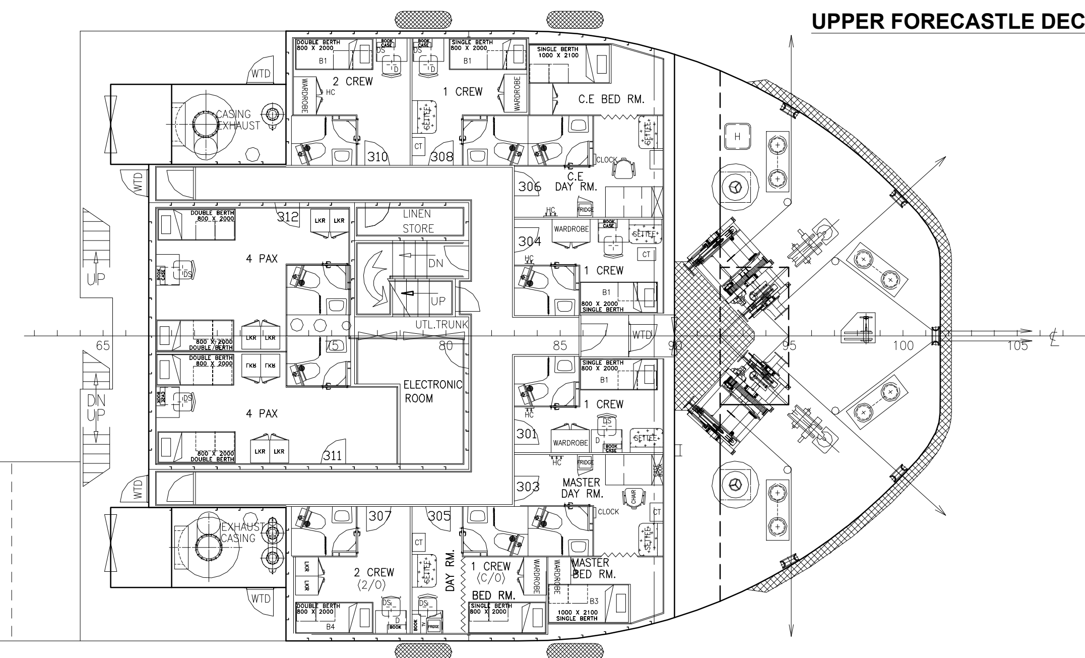
UPPER FORECASTLE DECK
