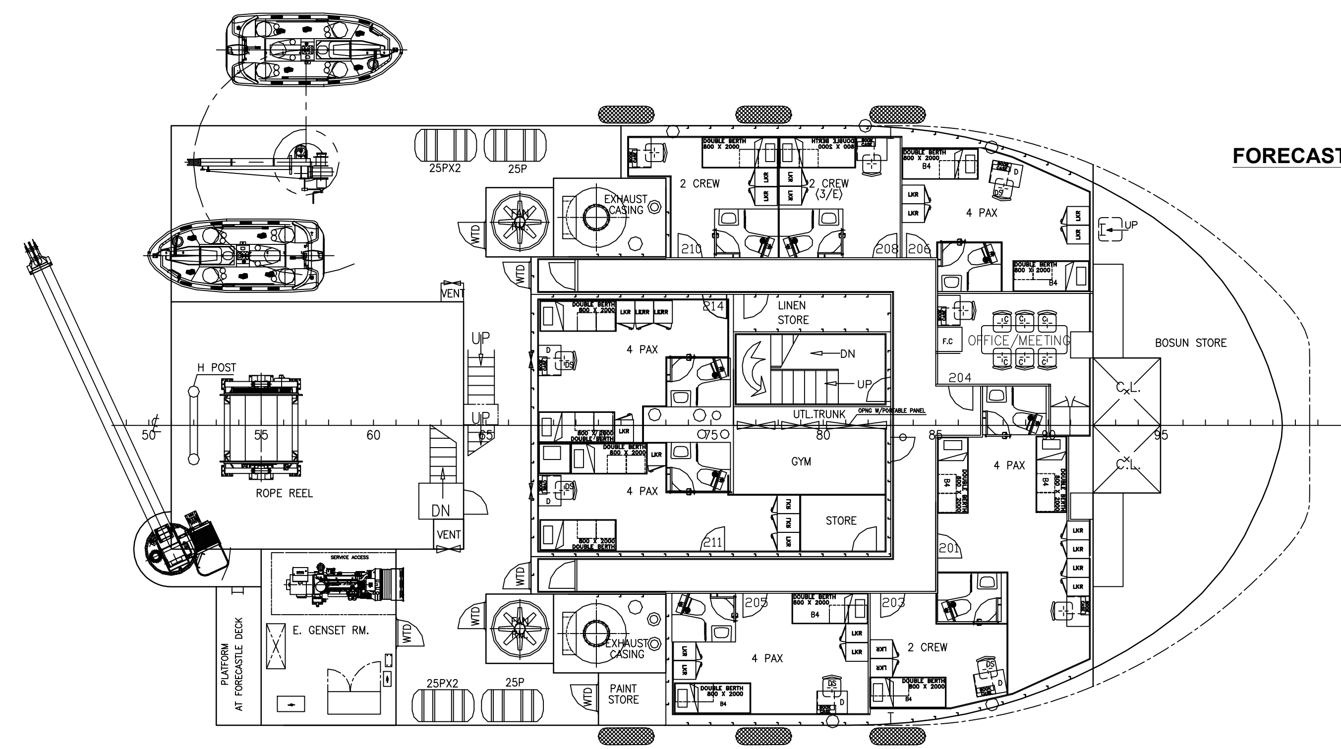
MAIN DECK PLAN
