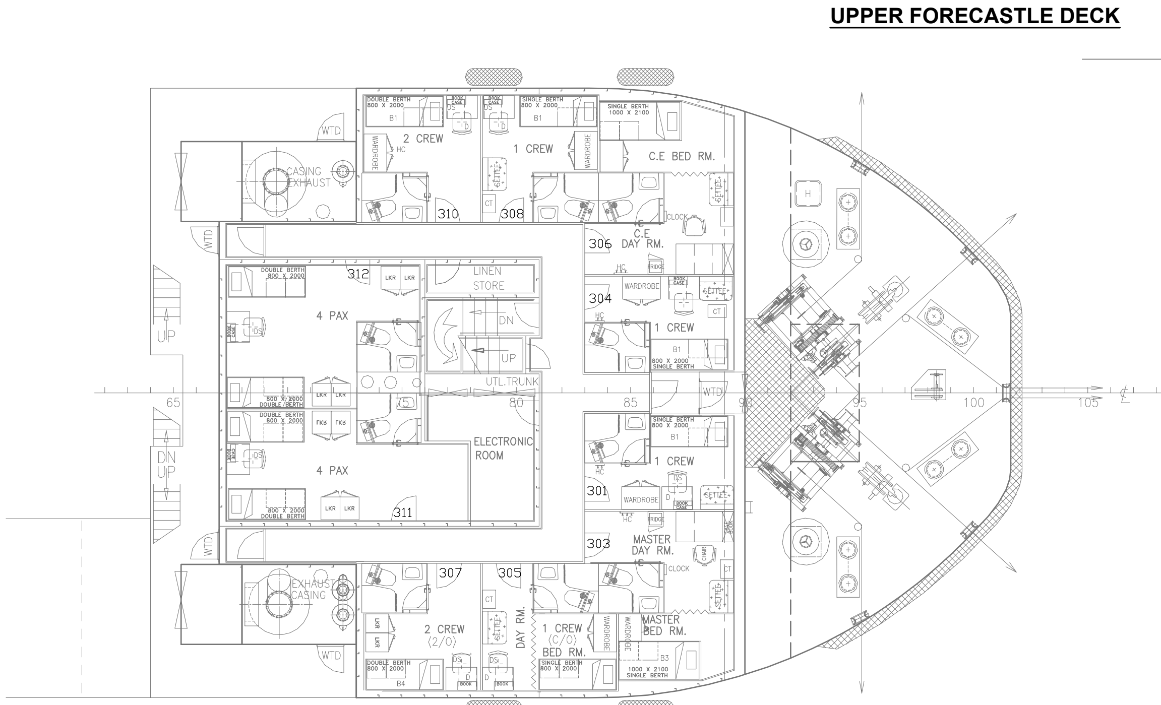
UPPER FORECASTLE DECK
